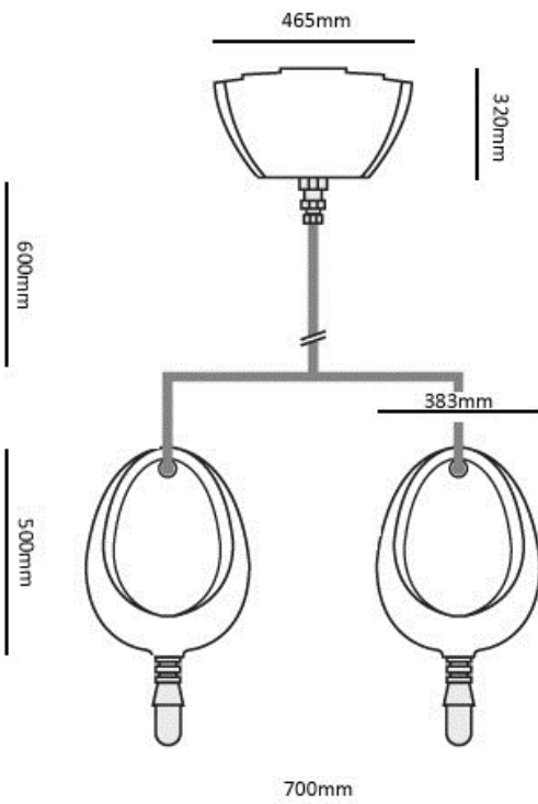
Coronus 2 Bowl Exposed Urinal Set
