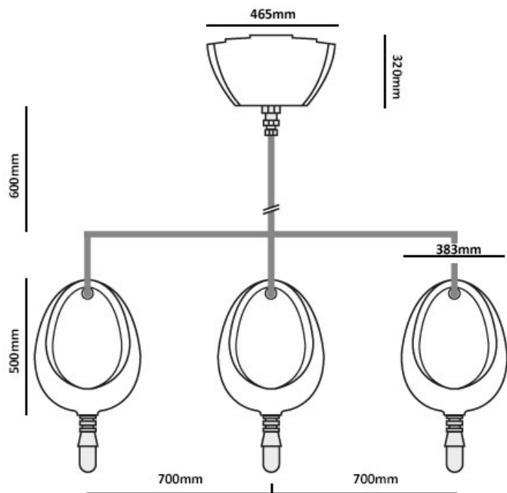
Coronus 3 Bowl Exposed Urinal Set
