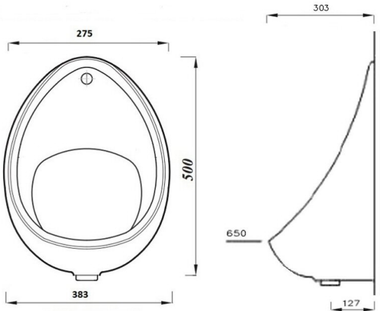
Coronus Urinal Bowl
